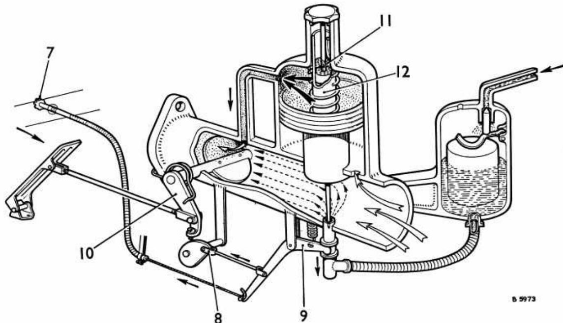
Fig. 2. Additions to the basic design (theoretical)
