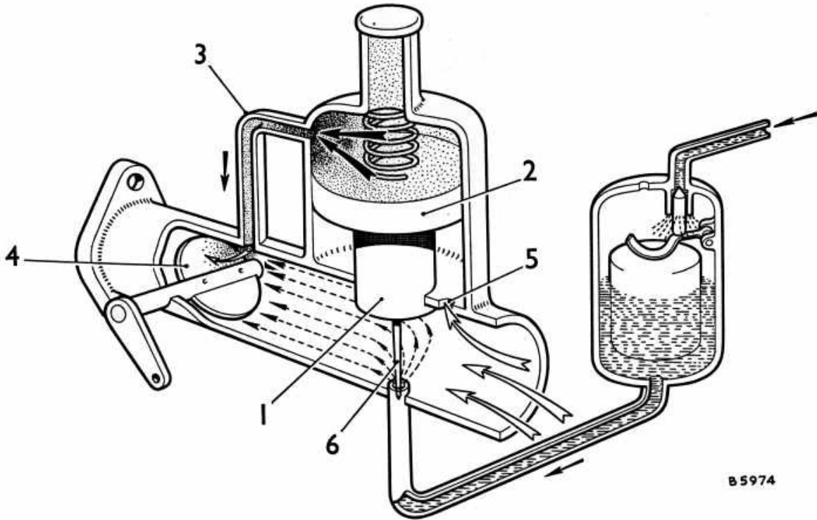
Fig. 1. The S.U. carburettor—basic construction (theoretical)
